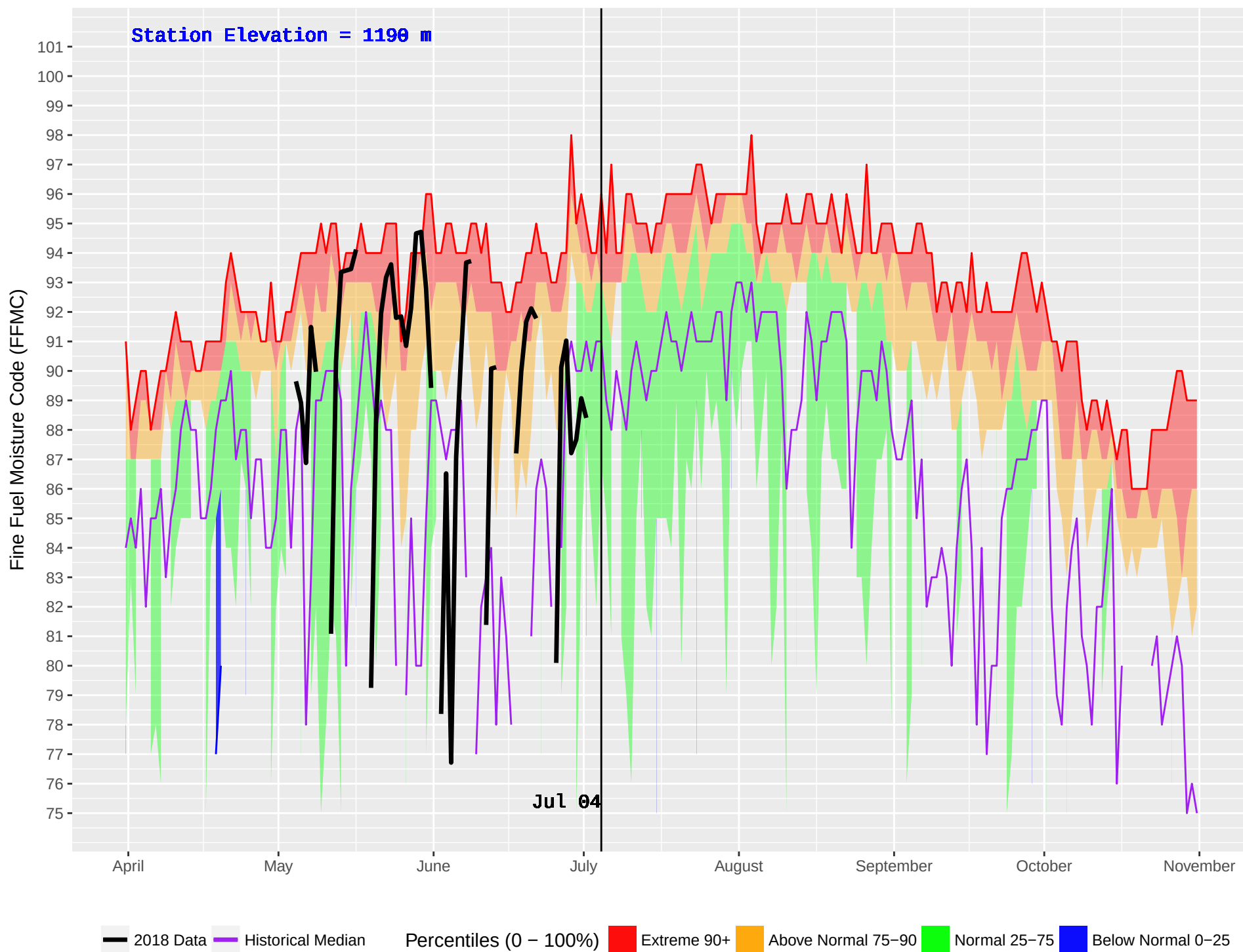
EMILY CREEK (425) : Historical (2002–2016) and Current (2018) Noon Fine Fuel Moisture Code (FFMC)
